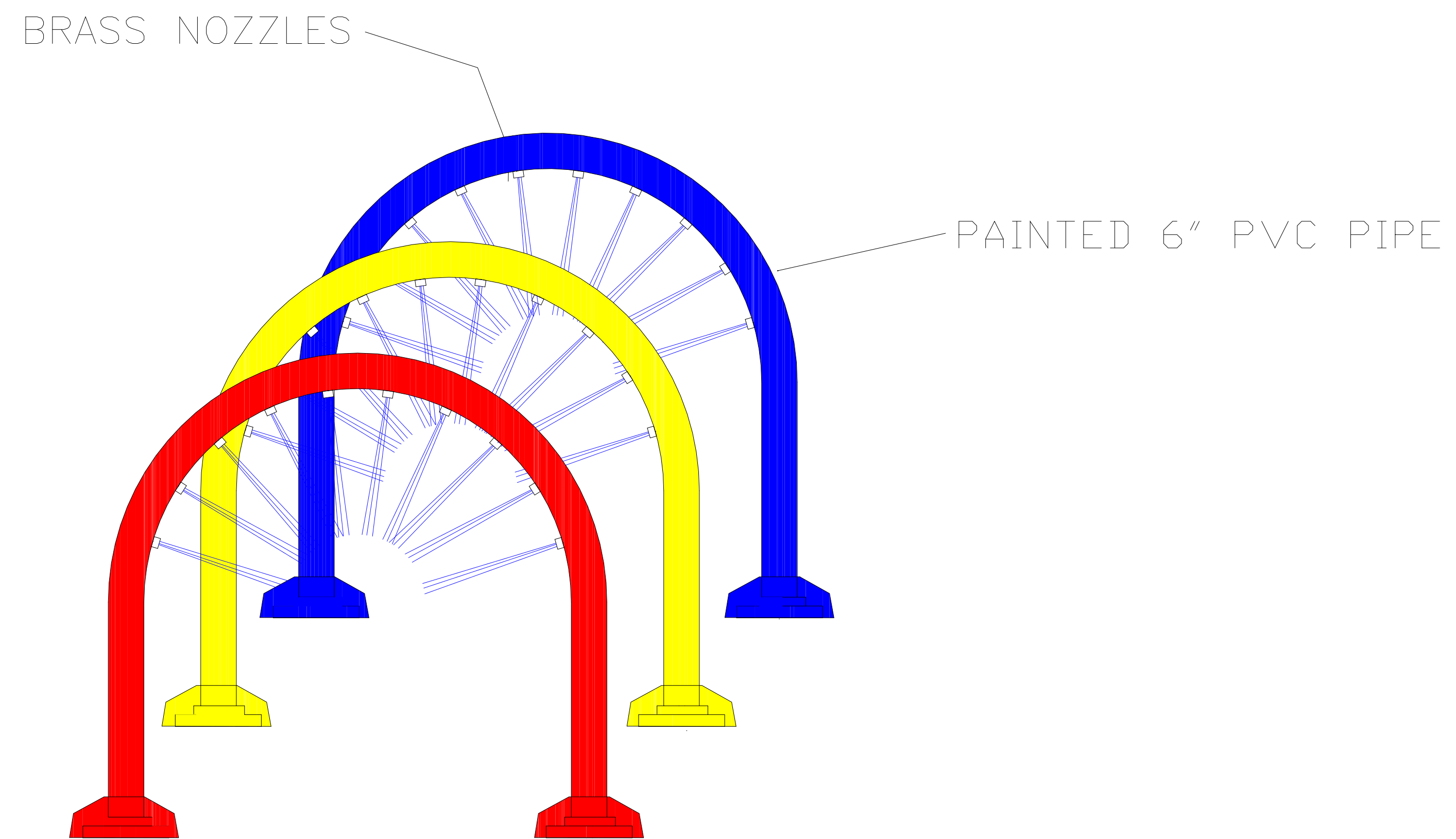
TYPICAL INSTALLATION
